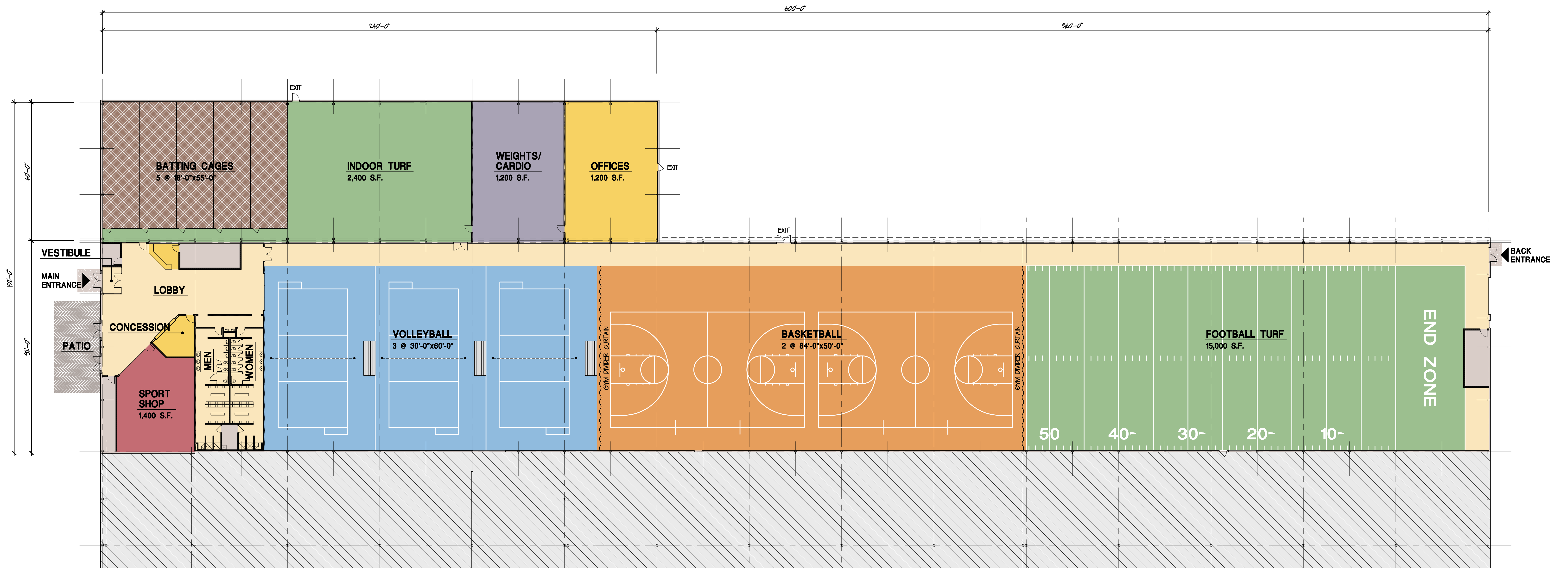
FLOOR PLAN SCALE: 1" = 20'-0"
